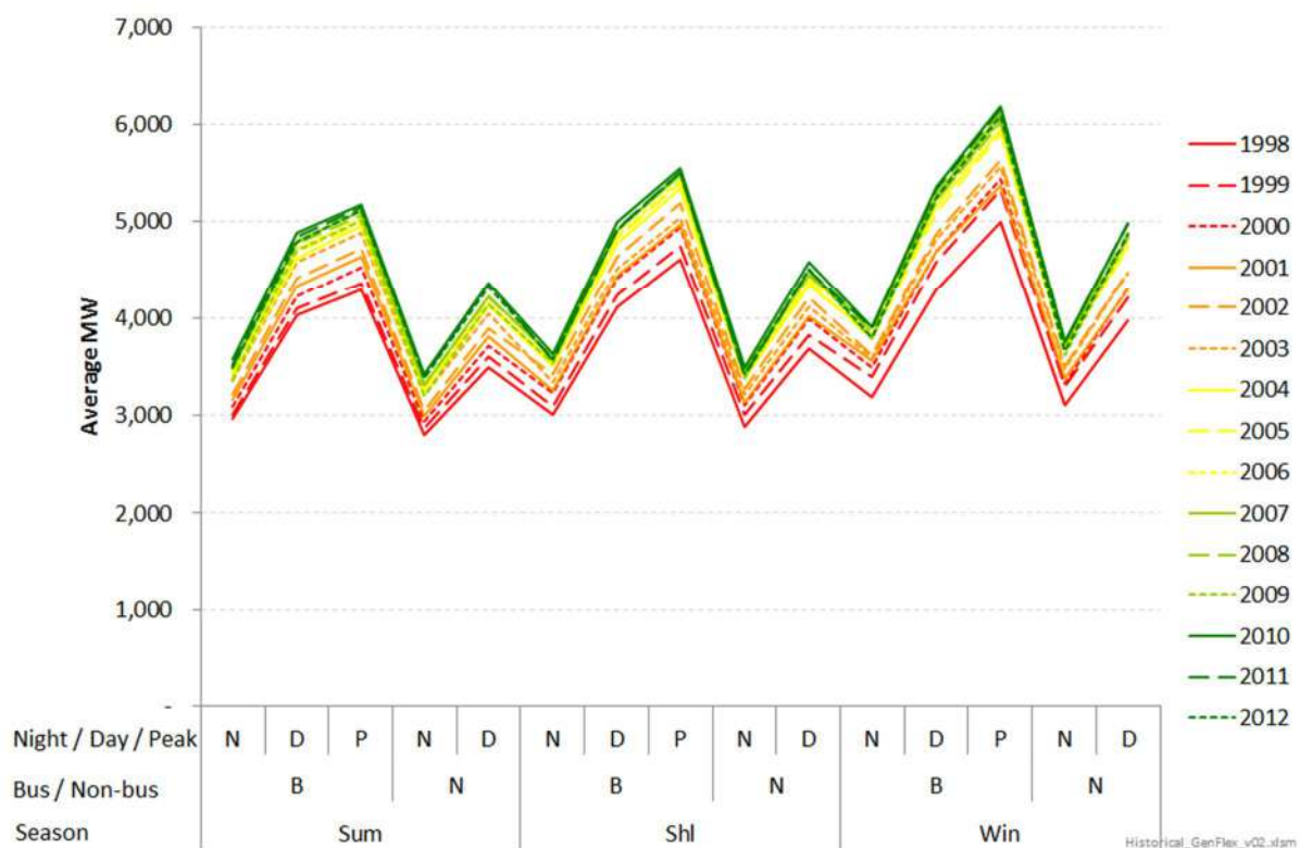
Figure 83: Average demand for different times of the day and year
