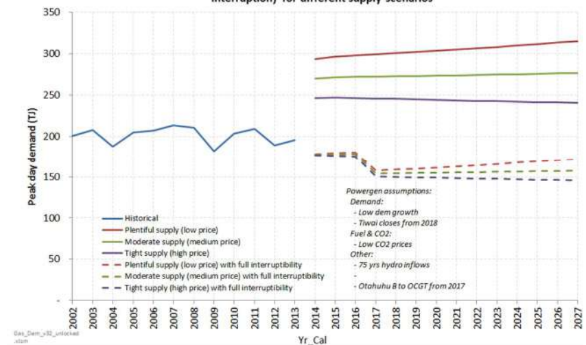
Projections of prudent peak day demand for All load North of Mokau (with and without interruption) for different supply scenarios
