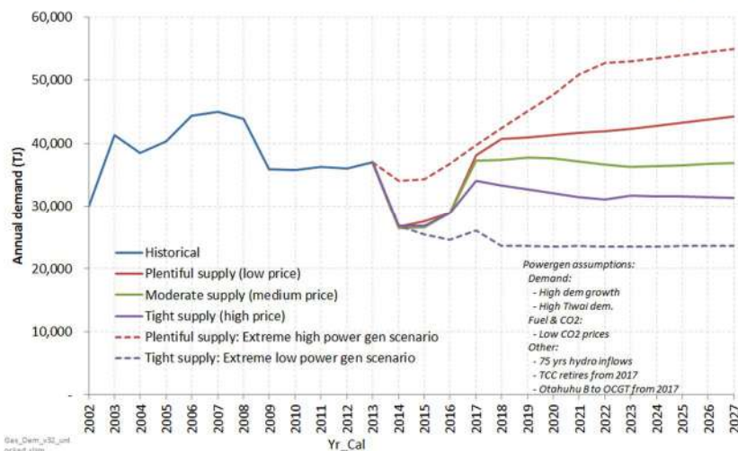
Projections of annual demand for Vector Tx 'North' system for different supply scenarios (TJ)
