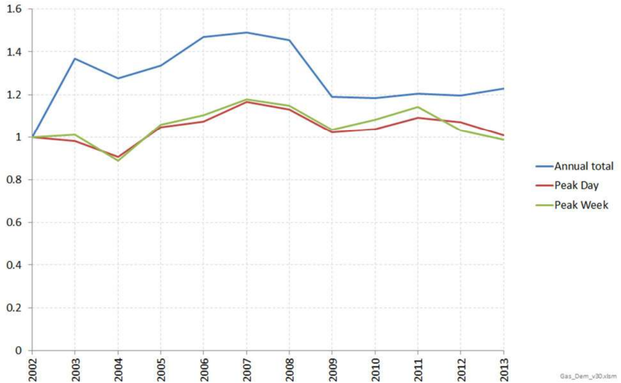
Figure 72: Relative movements in annual and peak demand for the North system
