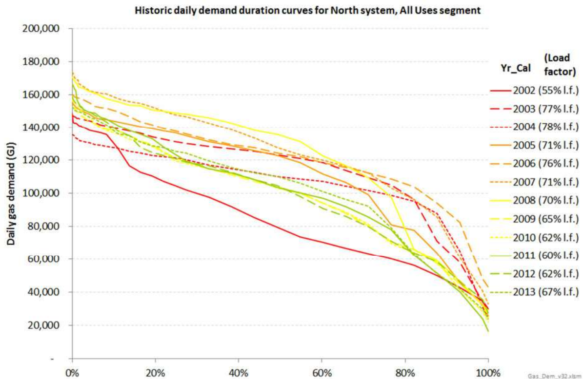
Figure 103: Duration curves of historical total daily gas demand on Vector North system
