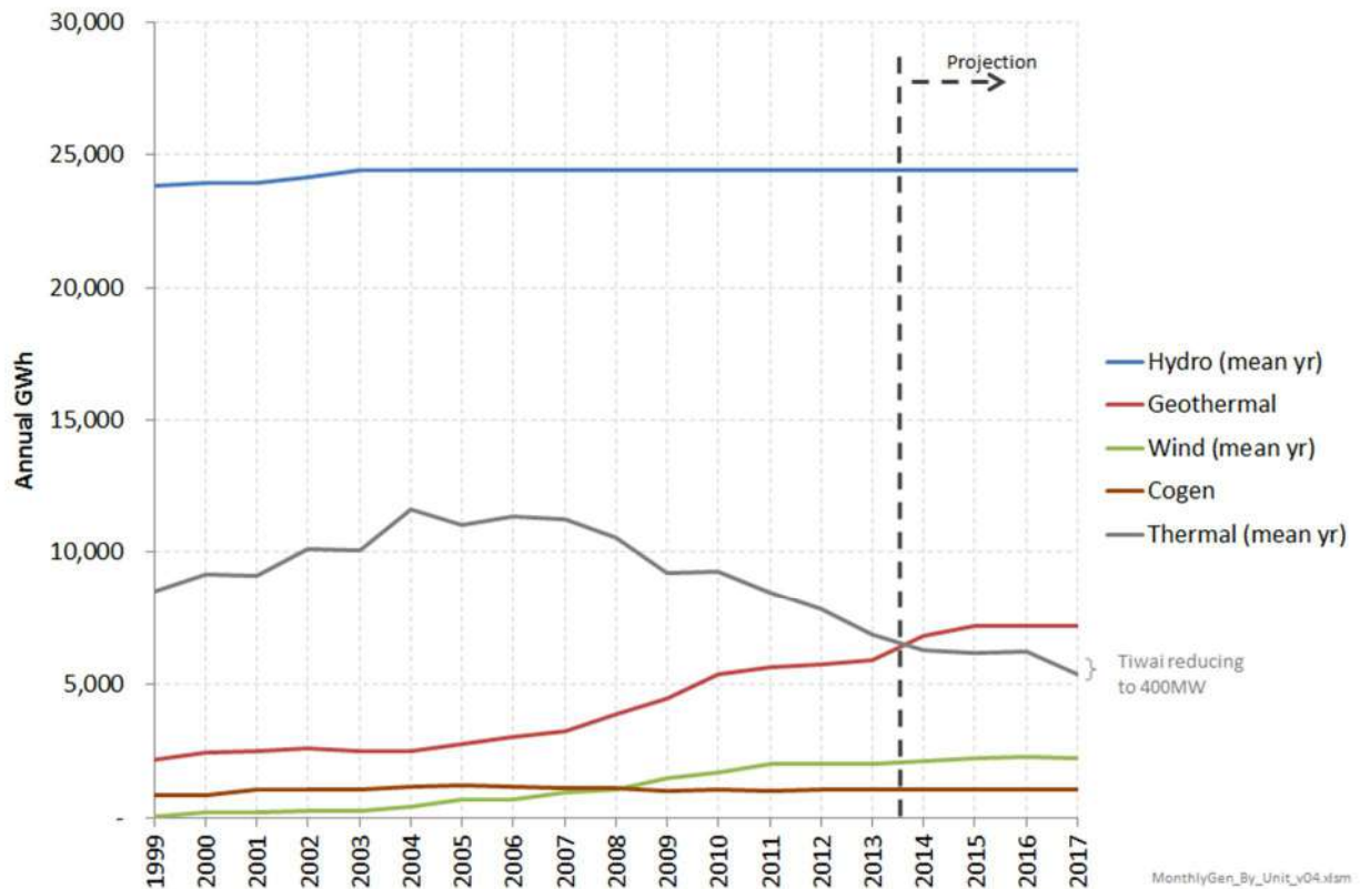
Figure 39: Historical and projected mean hydro-year generation from different types of generator – line graph
