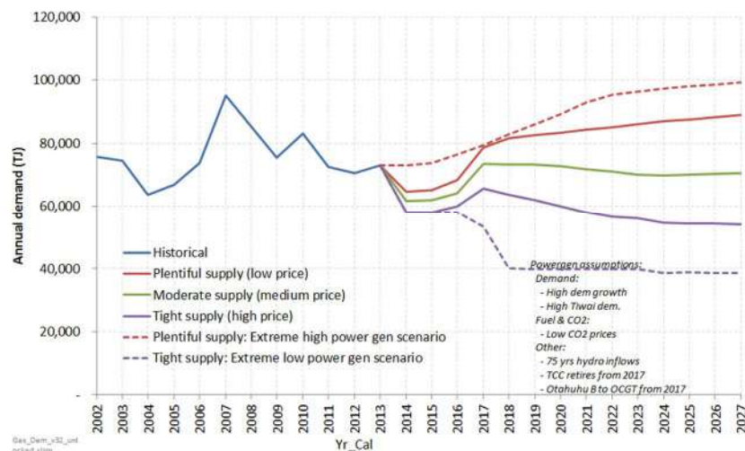
Projections of annual demand for All load North of Mokau for different supply scenarios (TJ)
