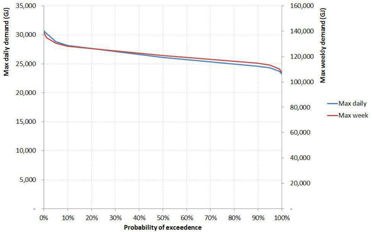
Figure 102: Example of probabilities of differing levels of peak day and peak week demand for the Non-TOU sector for the North system for 2012
