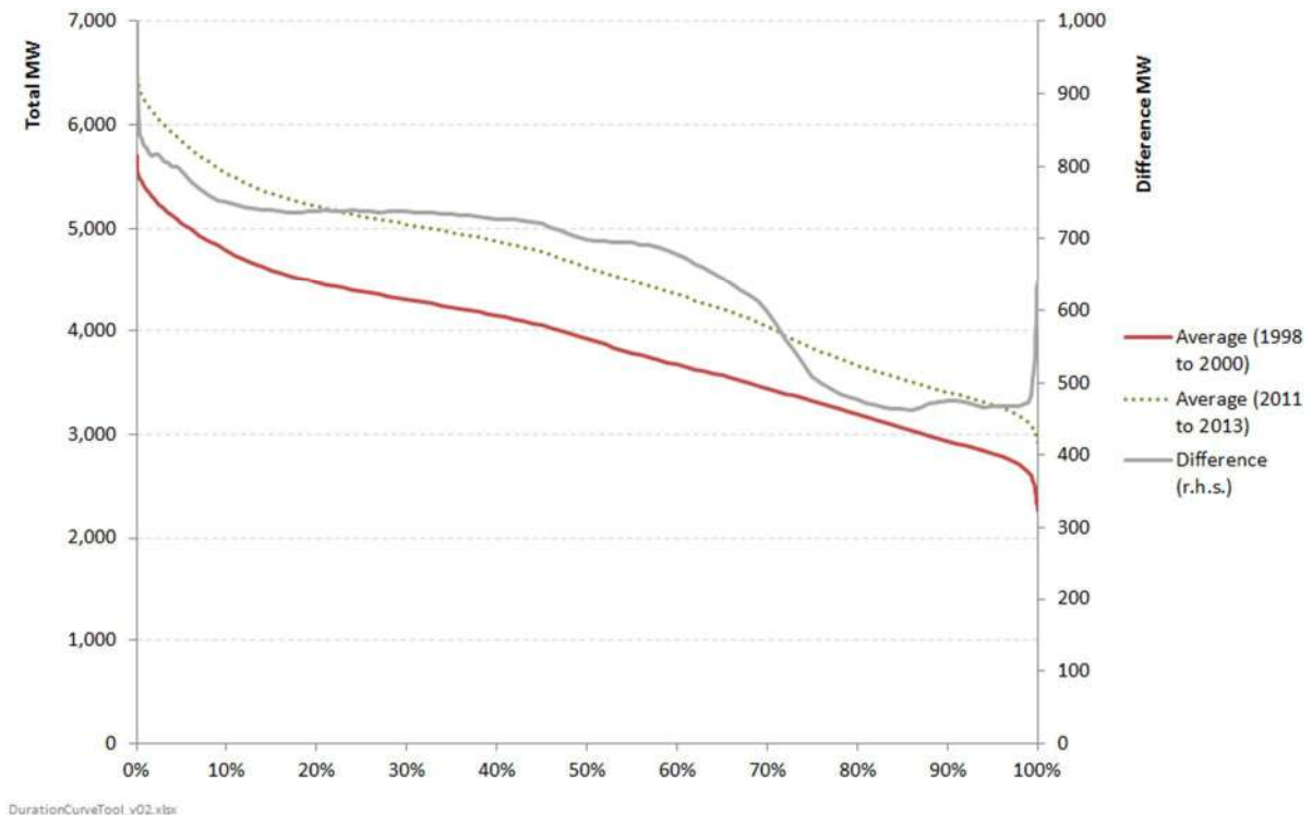
Figure 43: Historical change in the New Zealand electricity load duration curve
