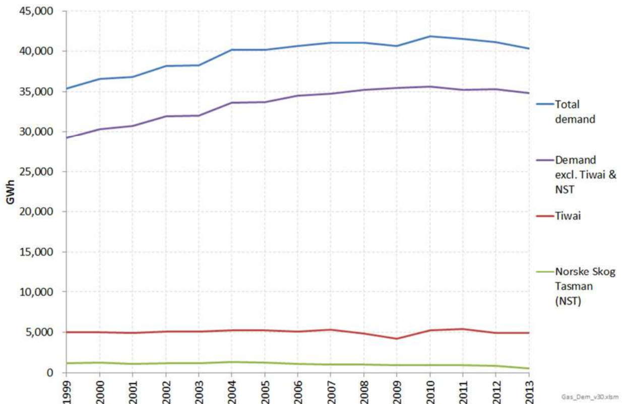
Figure 36: Historical annual demand, splitting out the Tiwai and Norske Skog Tasman sites
