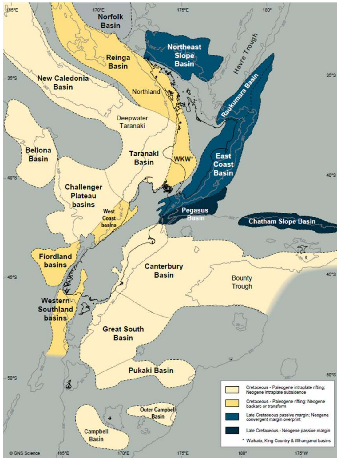
Figure 19: New Zealand petroleum basins
