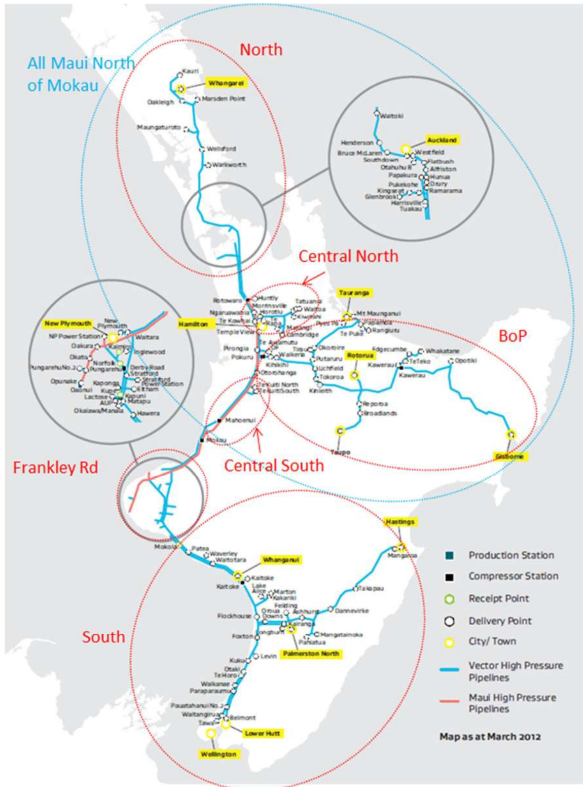
Figure 24: Gas transmission system, with regional definitions
