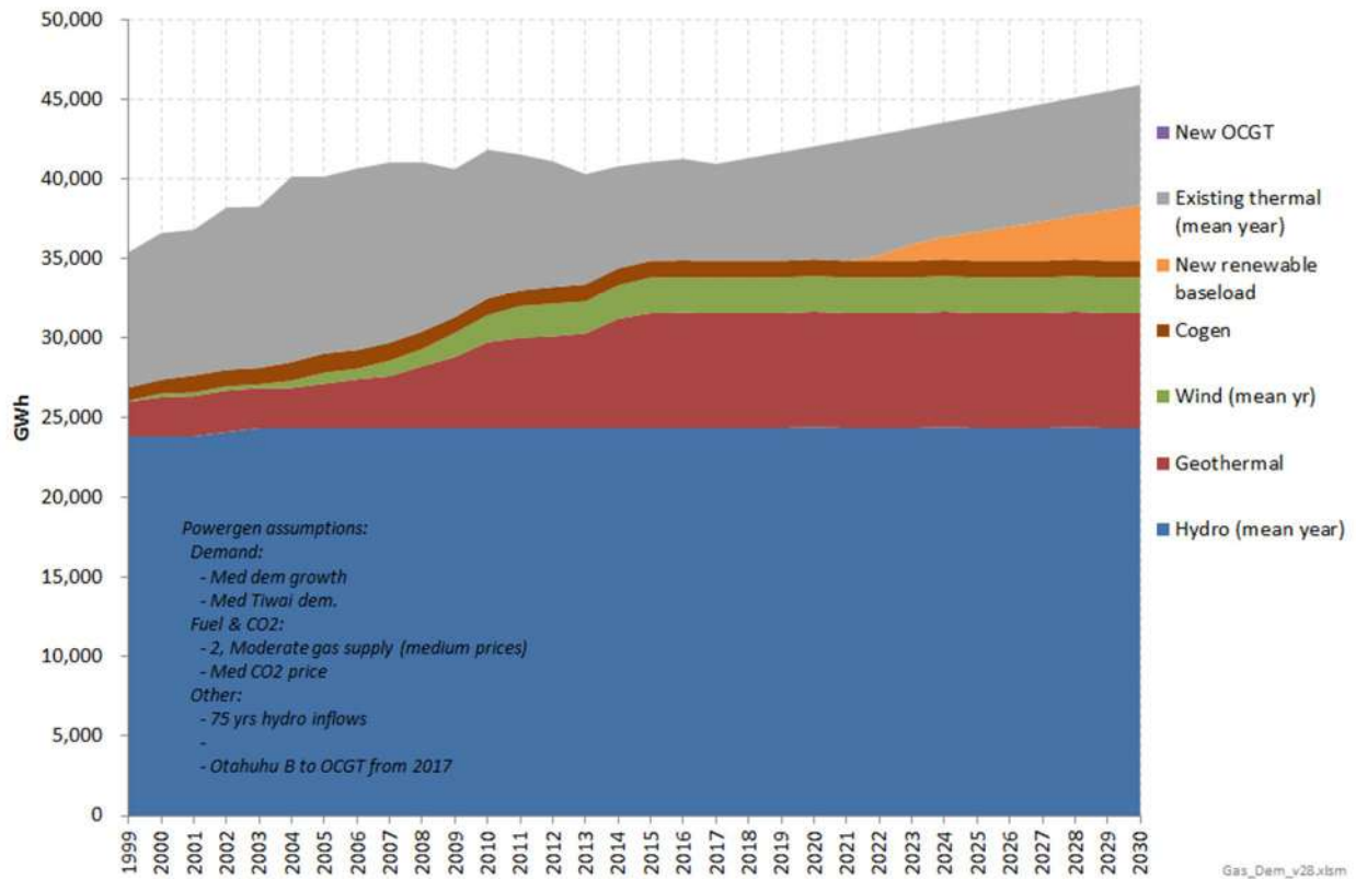
Figure 48: Projected mean year power generation from different types of generation - area graph
