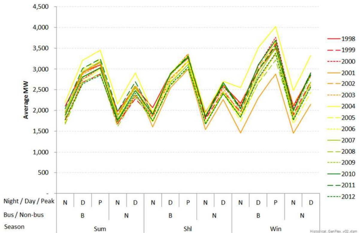
Figure 84: Average hydro generation for different times of the day and year
