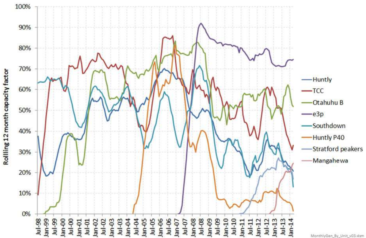
Figure 46: Historical capacity factor for key thermal power stations
