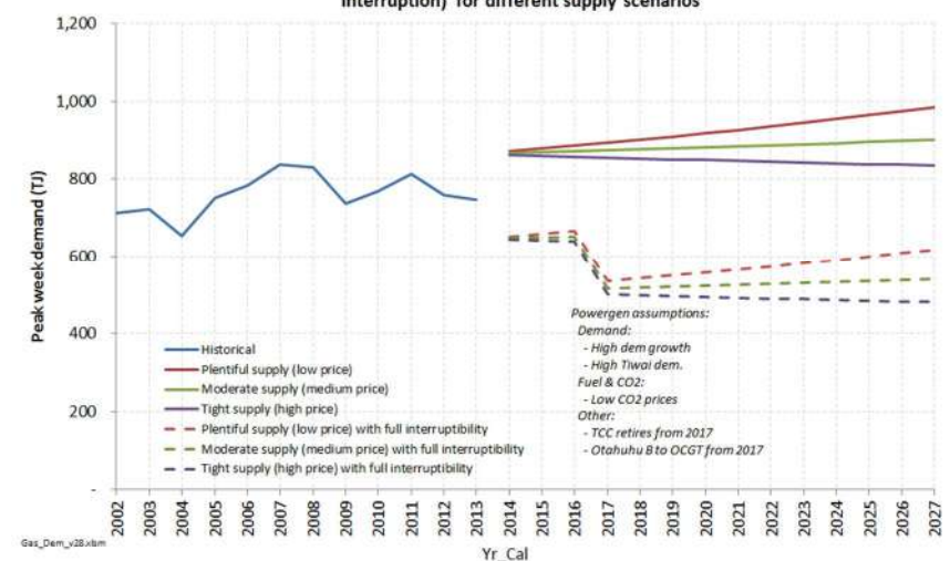
Projections of prudent peak week demand for Vector Tx 'North' system (with and without interruption) for different supply scenarios
