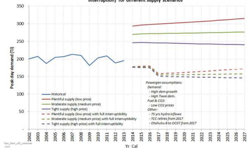
Projections of prudent peak day demand for All load North of Mokau (with and without interruption) for different supply scenarios
