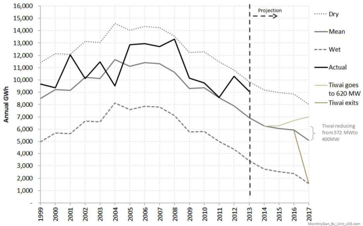
Figure 41: Historical and projected residual demand for thermal generation (excluding cogen) 56
