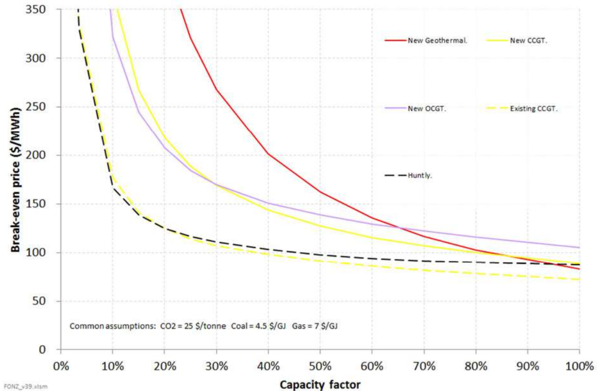
Figure 82: Costs of operation for different types of plant at different capacity factors for a hypothetical fuel and CO 2 market scenario 80
