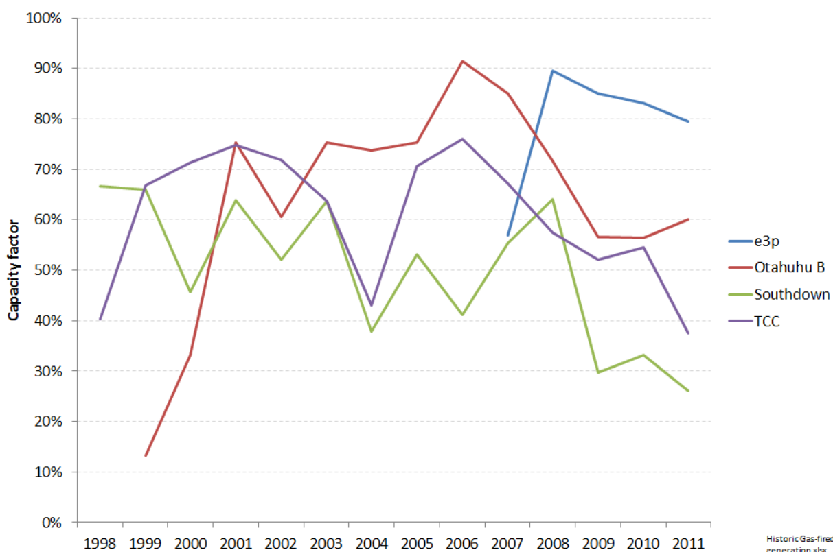
Figure 29: Historical capacity factors of gas-fired generation plant
