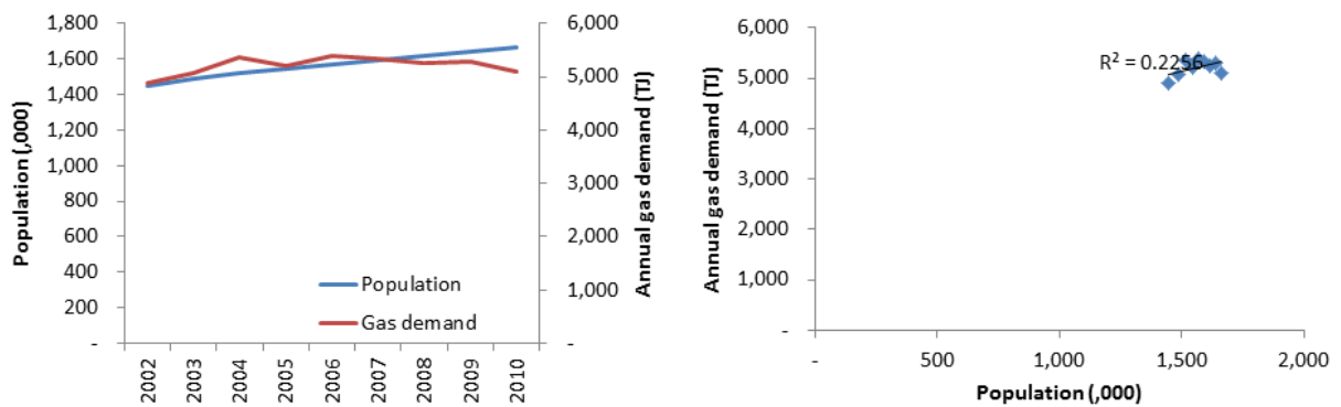
Correlation between Population and gas demand for Non-TOU sector in North system
