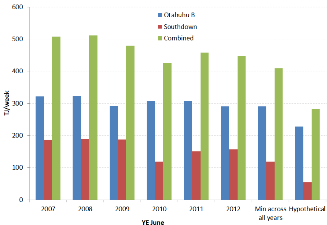
Figure 66: Illustration of potential scale of reduction in peak week gas consumption 66
