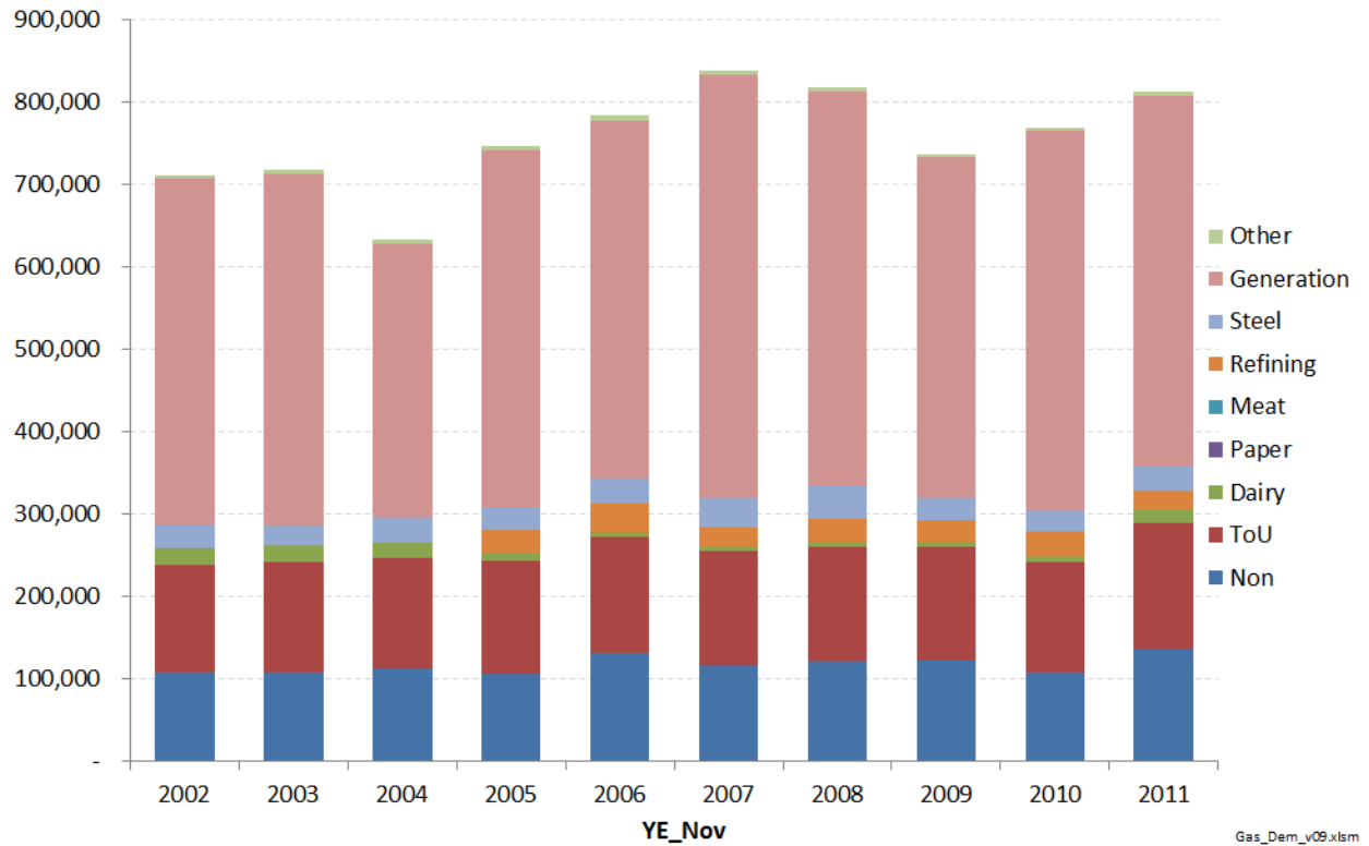
Figure 63: Historical sectoral composition of peak week demand for Vector North system (GJ)
