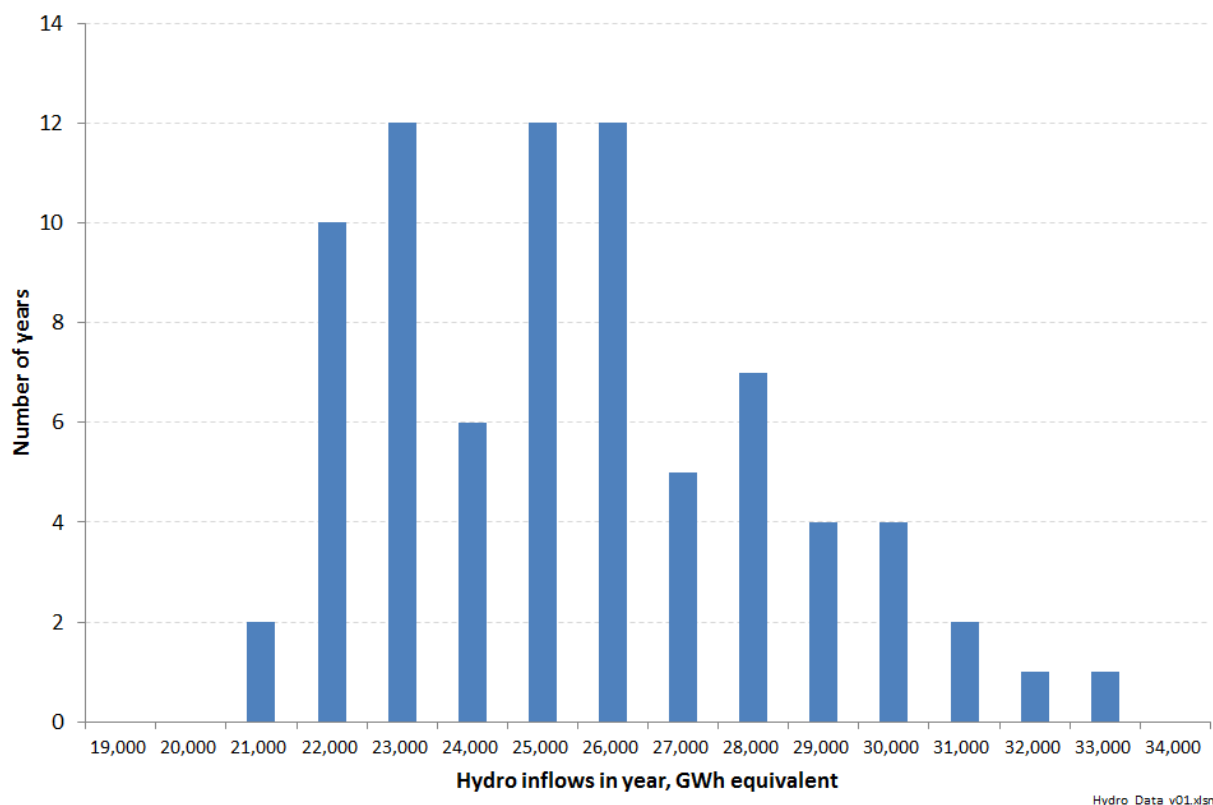
Figure 86: Historical frequency of occurrence of annual hydro inflows from 1932 to 2009
