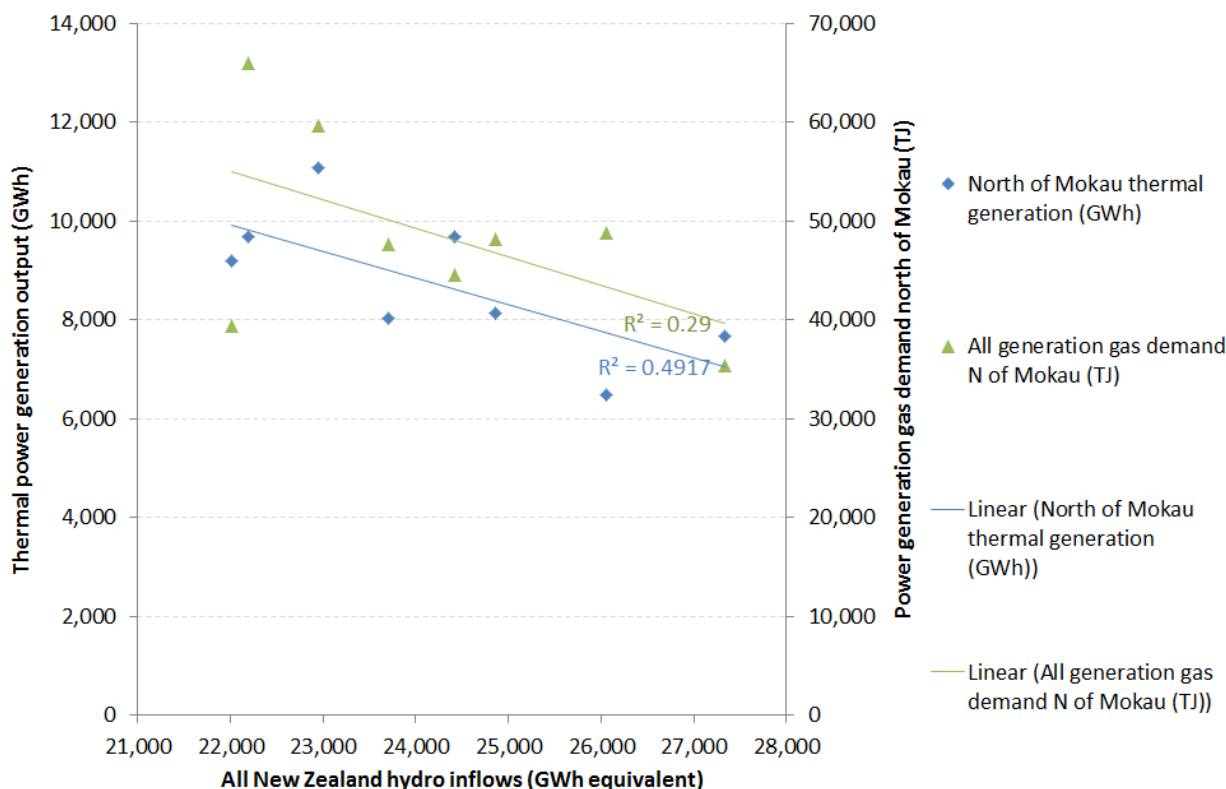
Figure 87: Comparison of hydro inflows with North of Mokou thermal power station generation and gas consumption for the years 2002 to 2009 (YE November basis)
