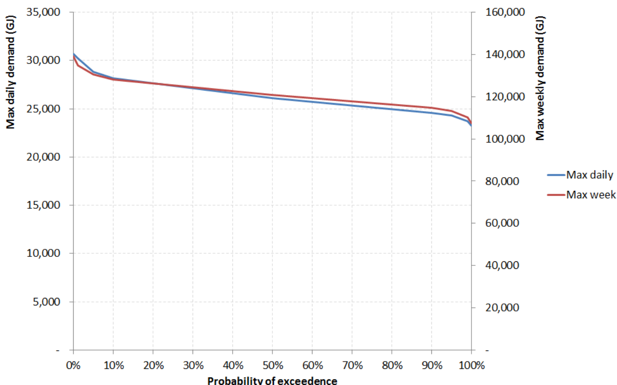
Figure 78: Example of probabilities of differing levels of peak day and peak week demand for the Non-TOU sector for the North system for 2012
