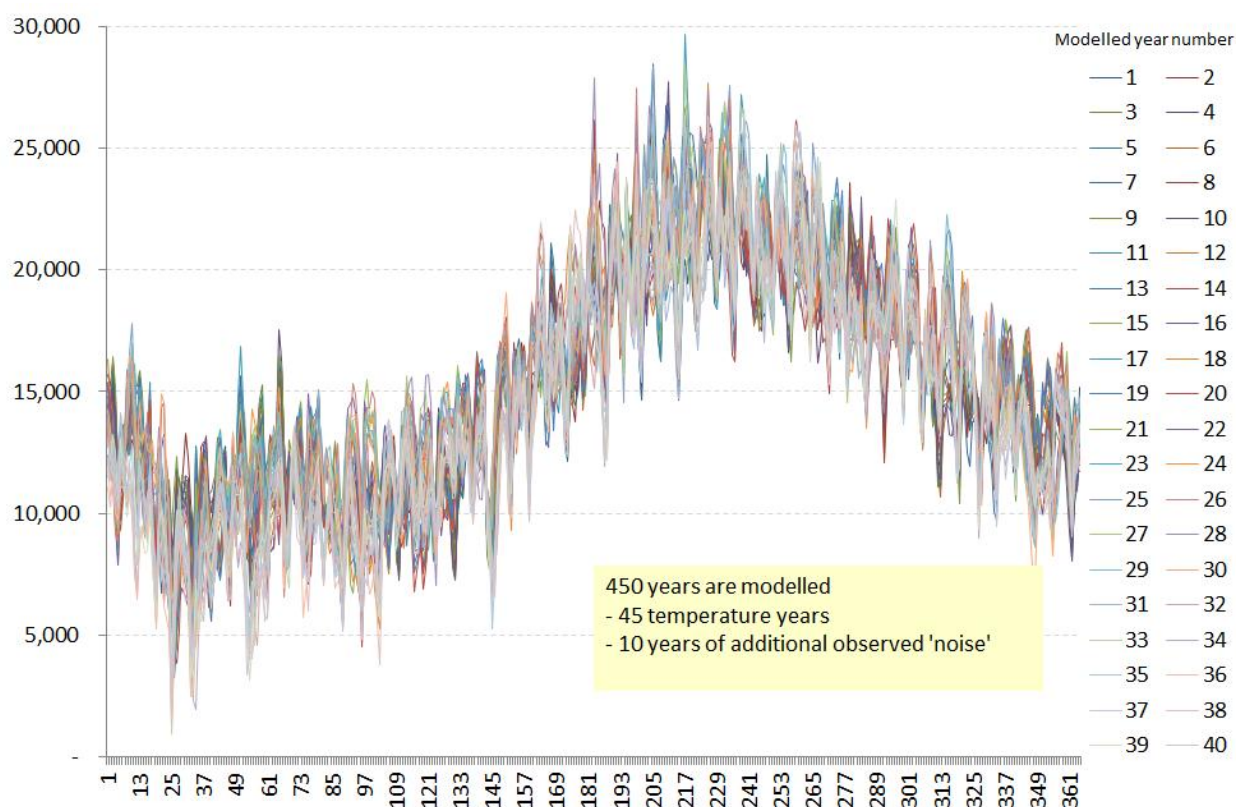
Figure 75: Example projections of daily Non-Tou demand for the North System for a sub-set of possible future years 73
