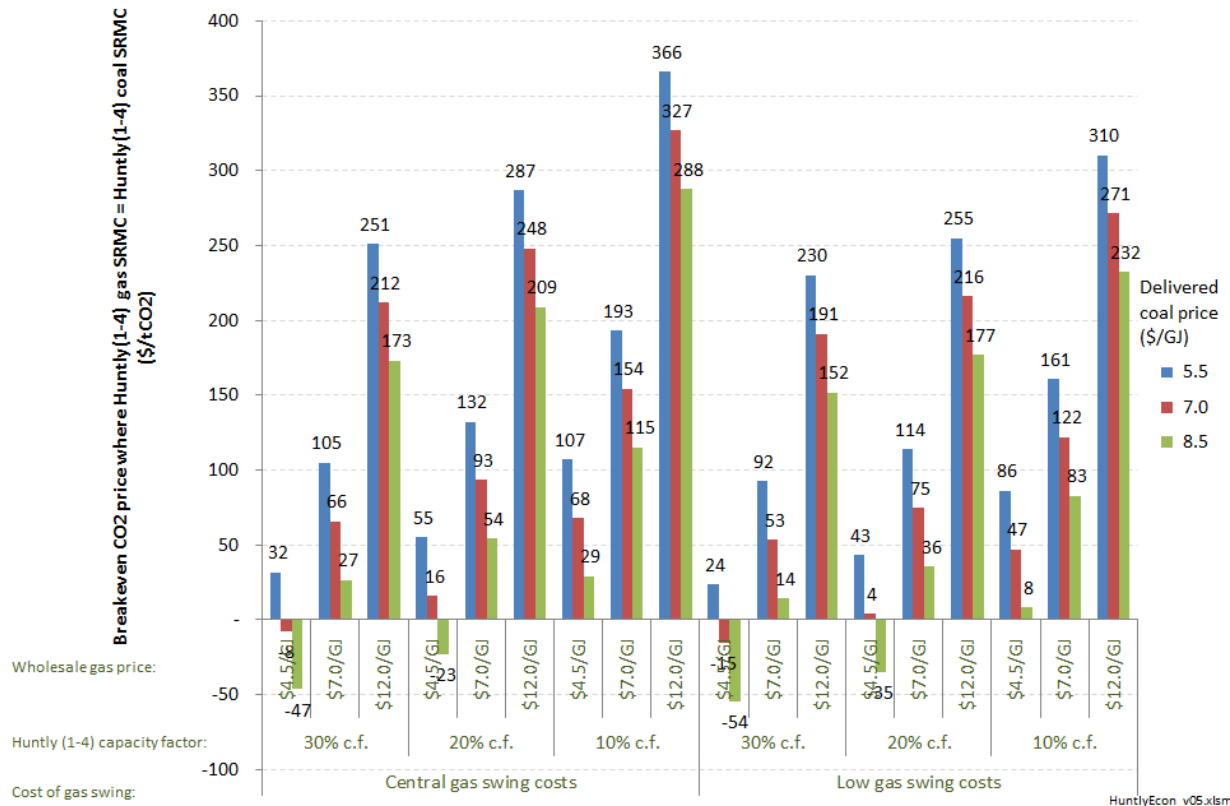
Figure 91: Estimation of the break-even CO 2 prices where the costs of burning coal and gas in Huntly (1-4) are equal
