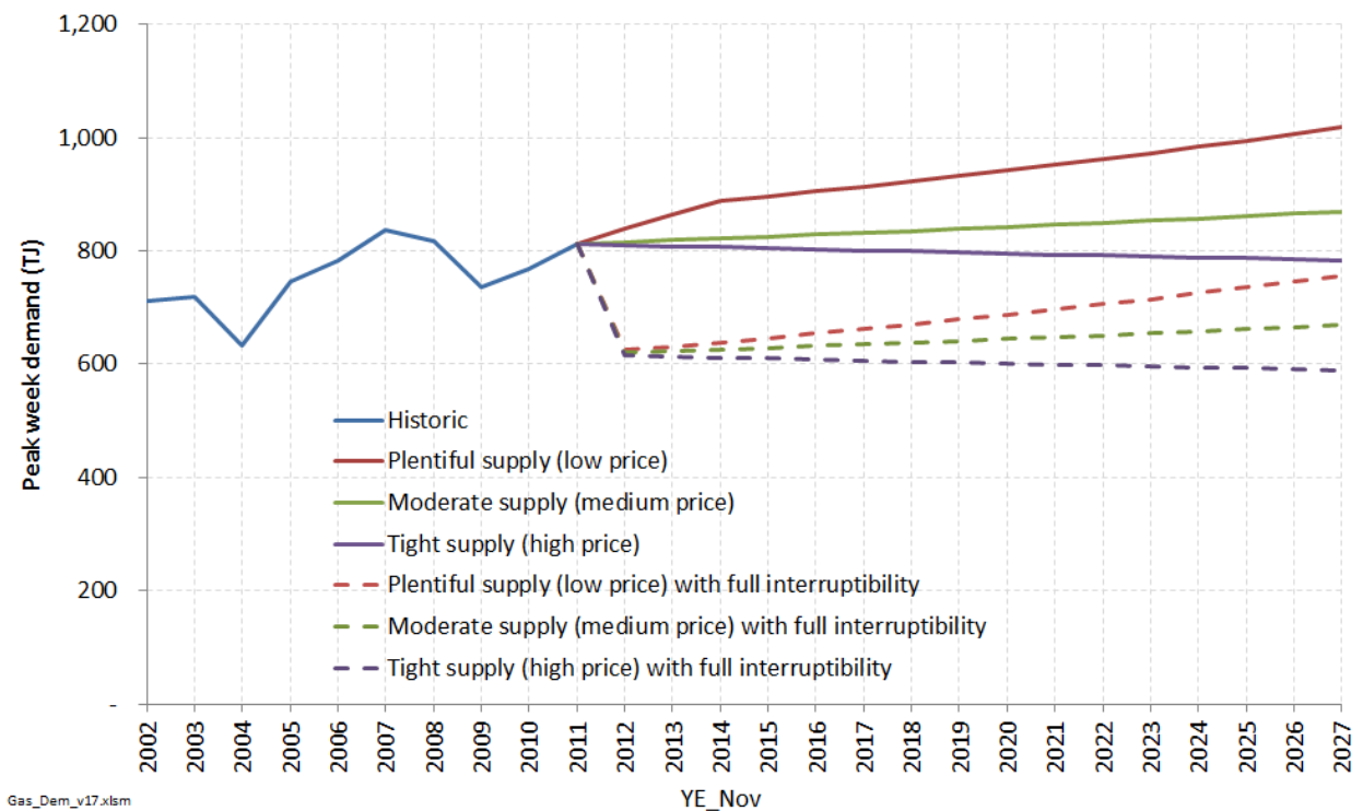
Figure 68: Projections of Vector North system peak week demand (with and without interruption) for different supply scenarios
