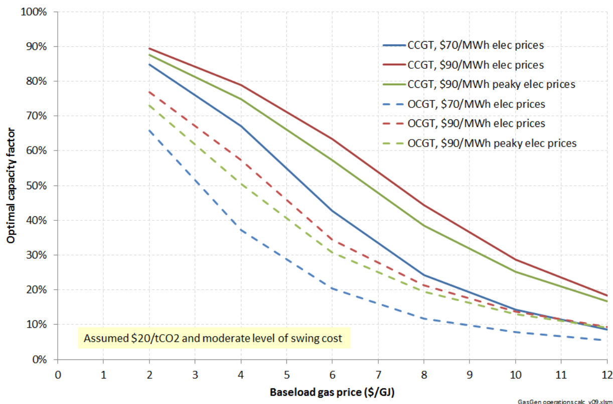
Figure 30: Simulation of different optimal gas-fired generator operating patterns in response to varying gas prices
