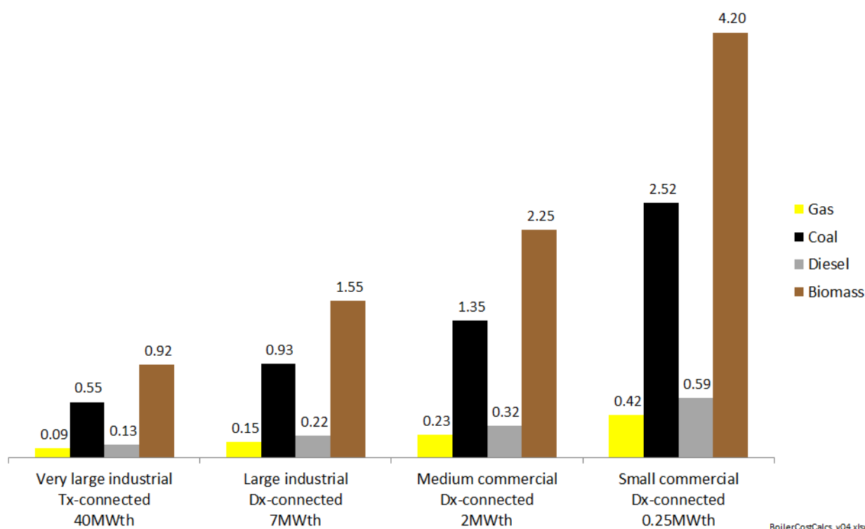
Figure 79: Estimated boiler capital costs for different sized intermediate process heat boilers ($m/MWth)
