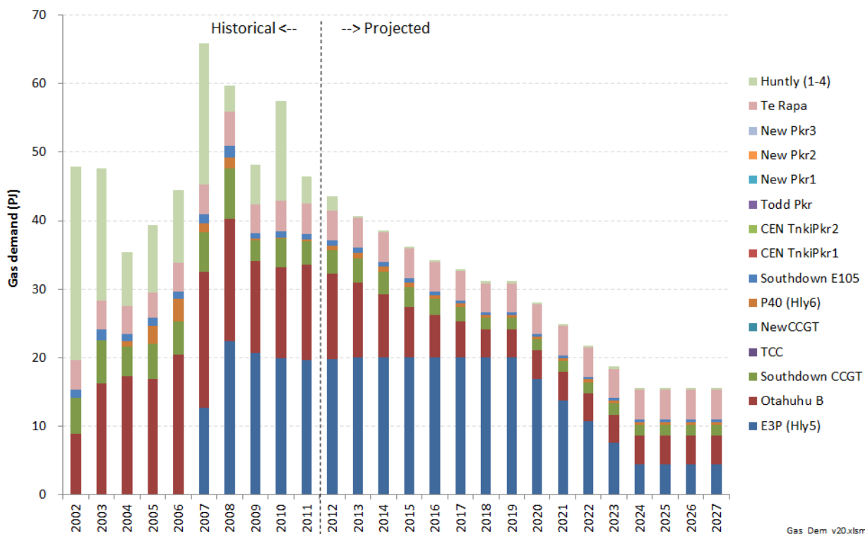
Figure 94: Historical and projected mean gas consumption from power stations located North of Mokau for the high gas price scenario
