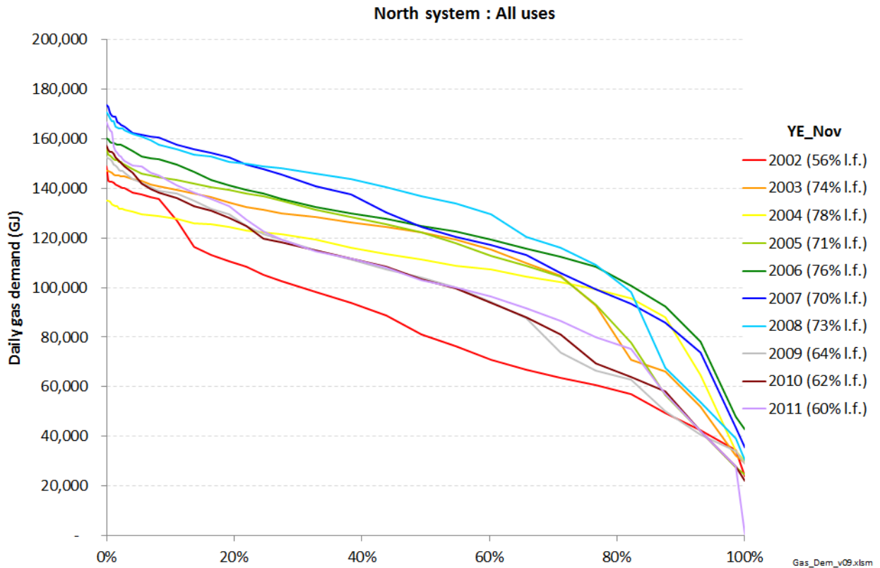
Figure 56: Duration curves of historical total daily gas demand on Vector North system
