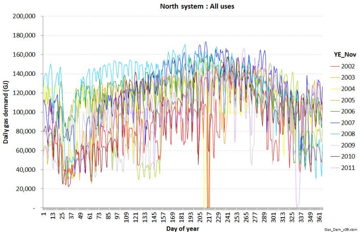
Figure 55: Historical total daily gas demand on Vector North system 62
