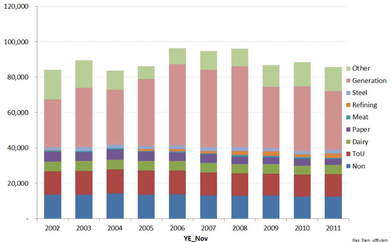
Figure 37: Historical consumption split by customer use across Vector transmission system (TJ) 53
