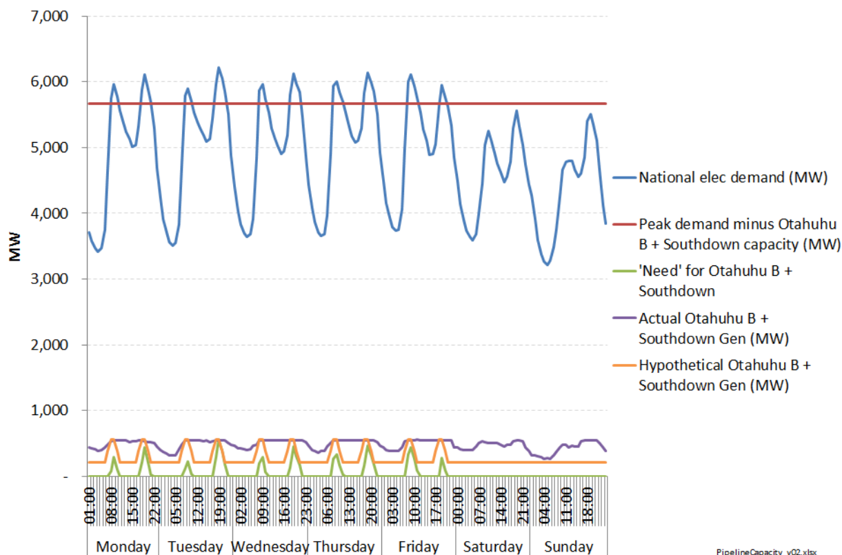
Figure 65: Simplified analysis of the potential for additional cycling of Auckland generators
