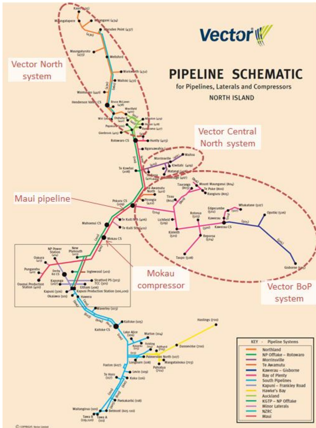
Figure 82: Pipeline schematic
