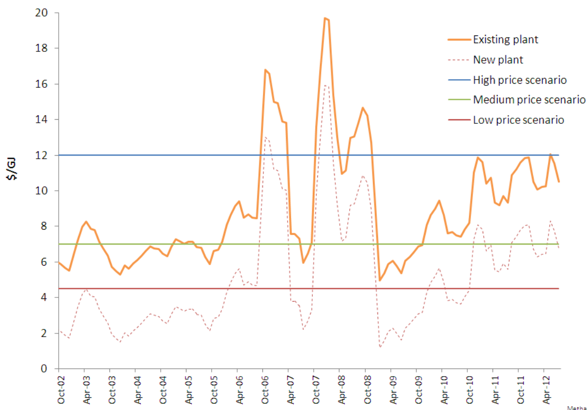
Figure 20: Estimated breakeven gas price for methanol manufacturing (nominal)
