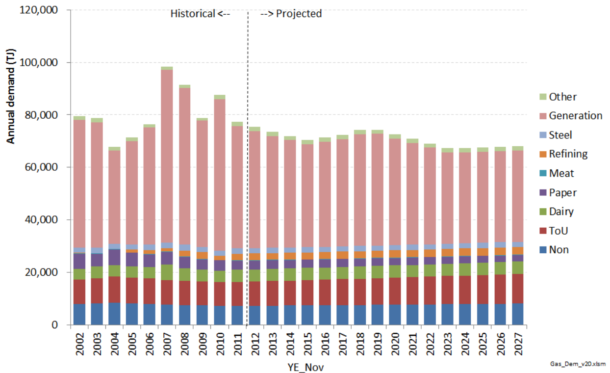
Figure 85: Historical and projected annual demand for different customer segments for all load north of Mokau for the Medium price scenario
