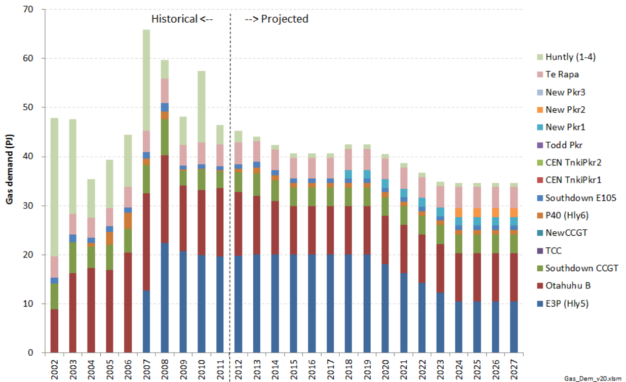
Figure 93: Historical and projected mean gas consumption from power stations located North of Mokau for the medium gas price scenario
