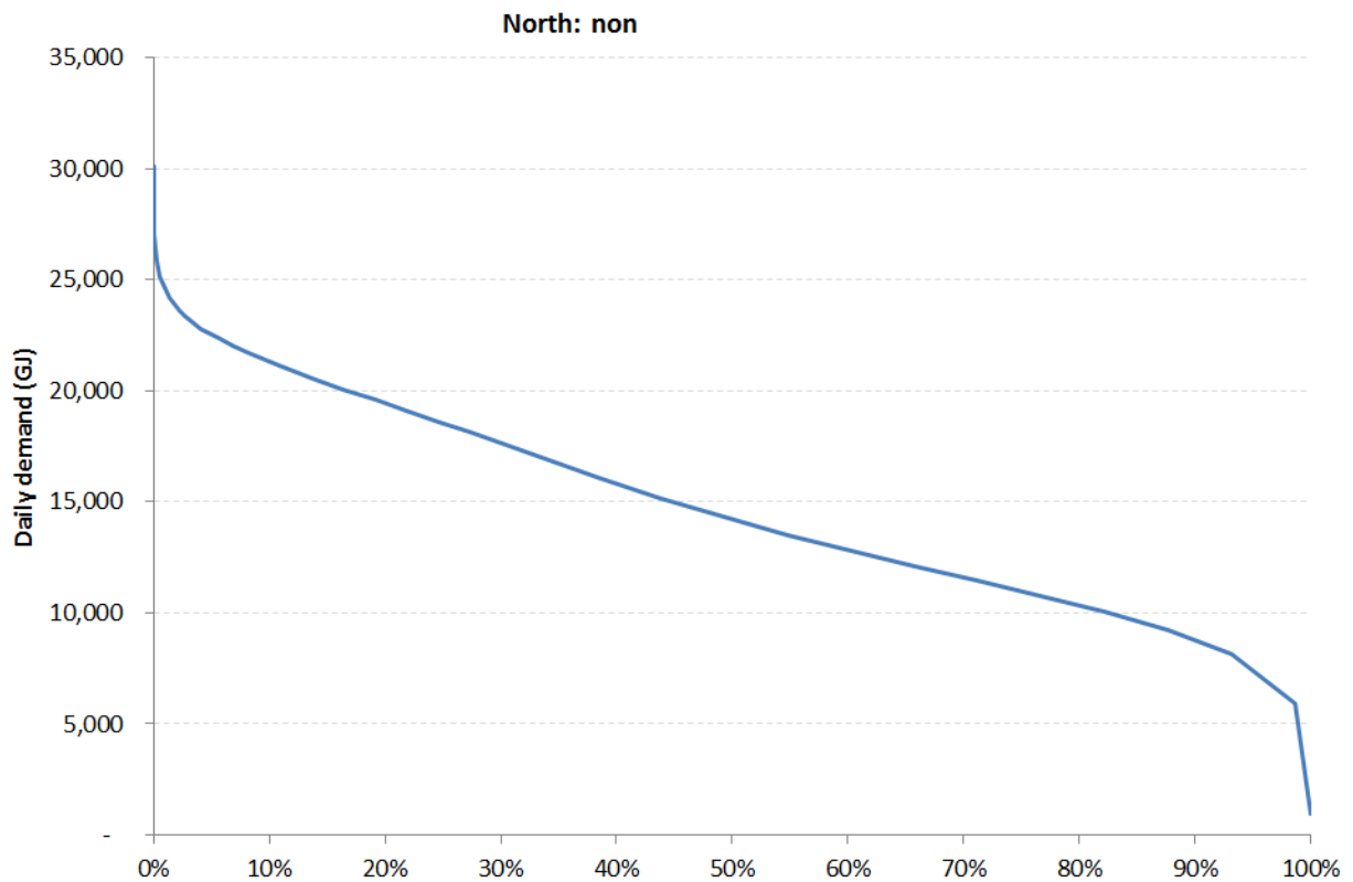
Figure 76: Duration curve of modelled gas demand for Non-Tou sector for North system over a 45 year time-frame
