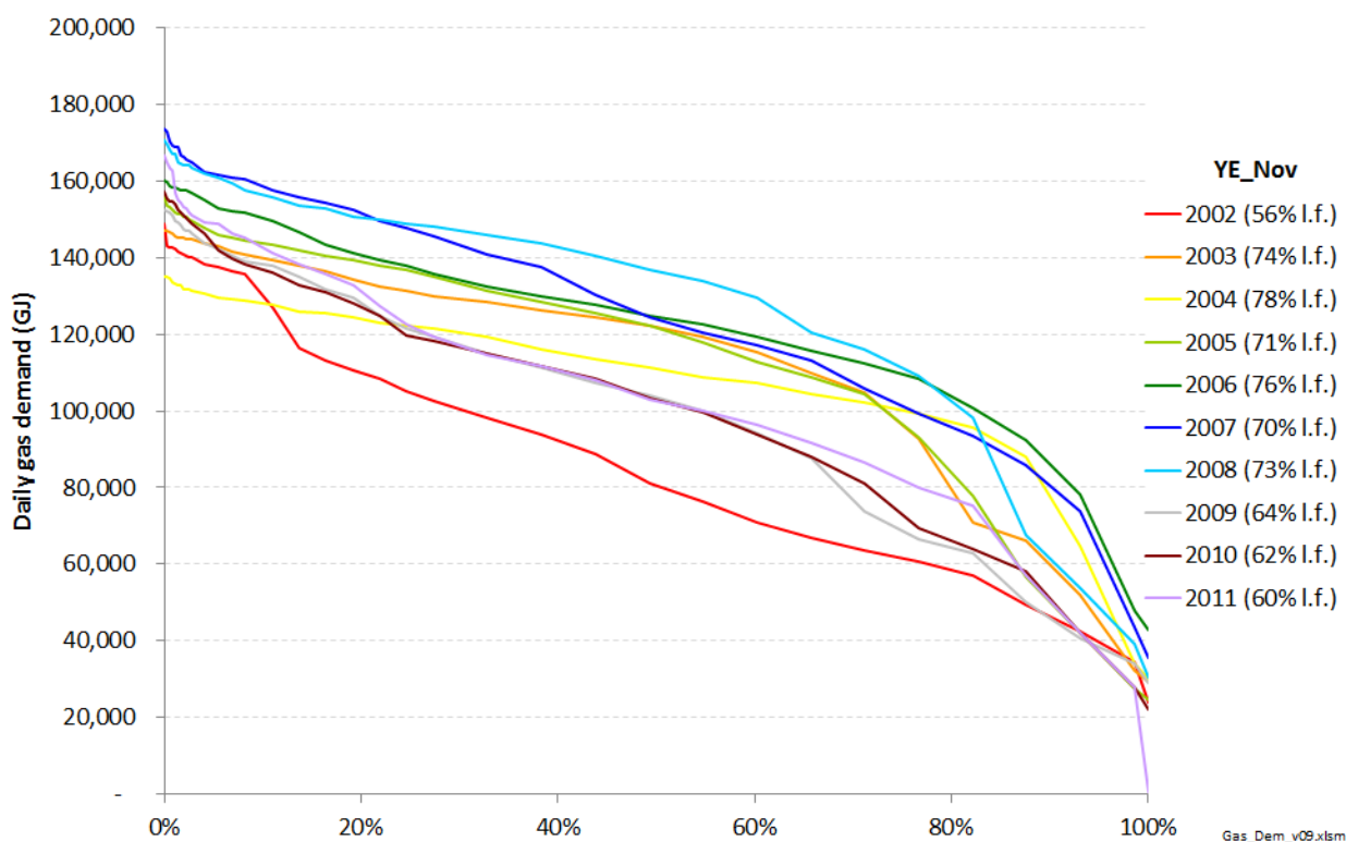
Figure 62: Duration curves of historical total daily gas demand on Vector North system
