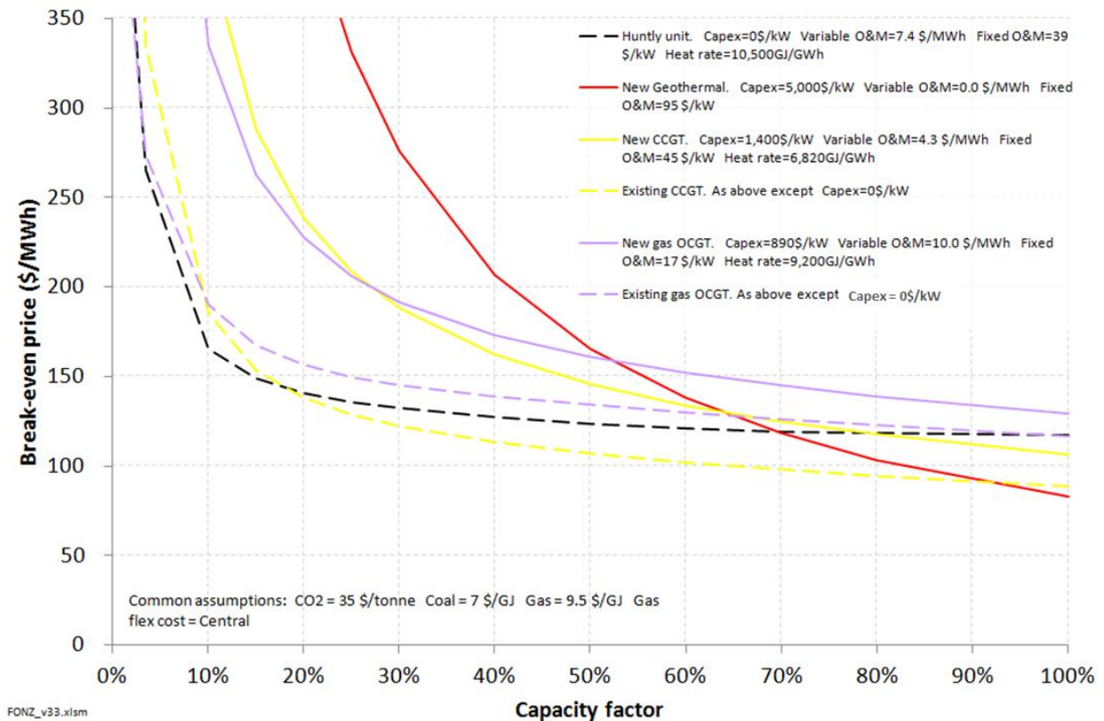
Figure 28: Generator cost curves
