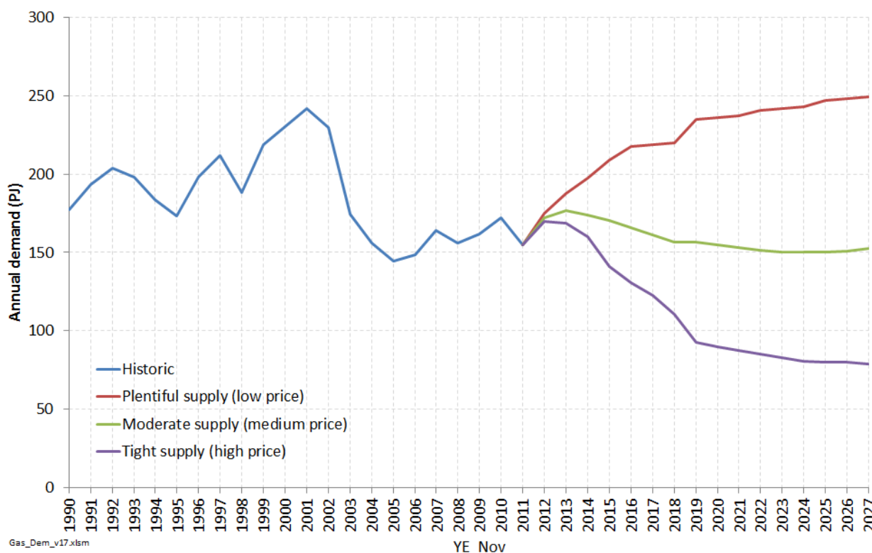
Figure 2: Projections of total New Zealand gas demand
