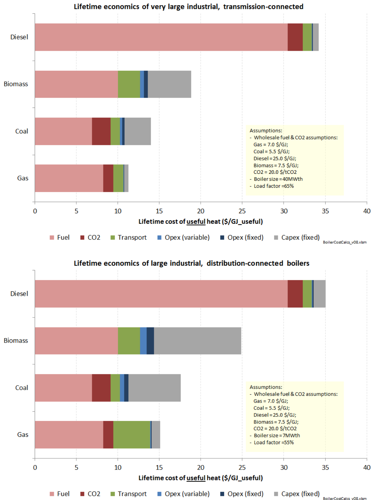
Figure 47: Illustration of the relative economics of new-build boilers for industrial process heat
