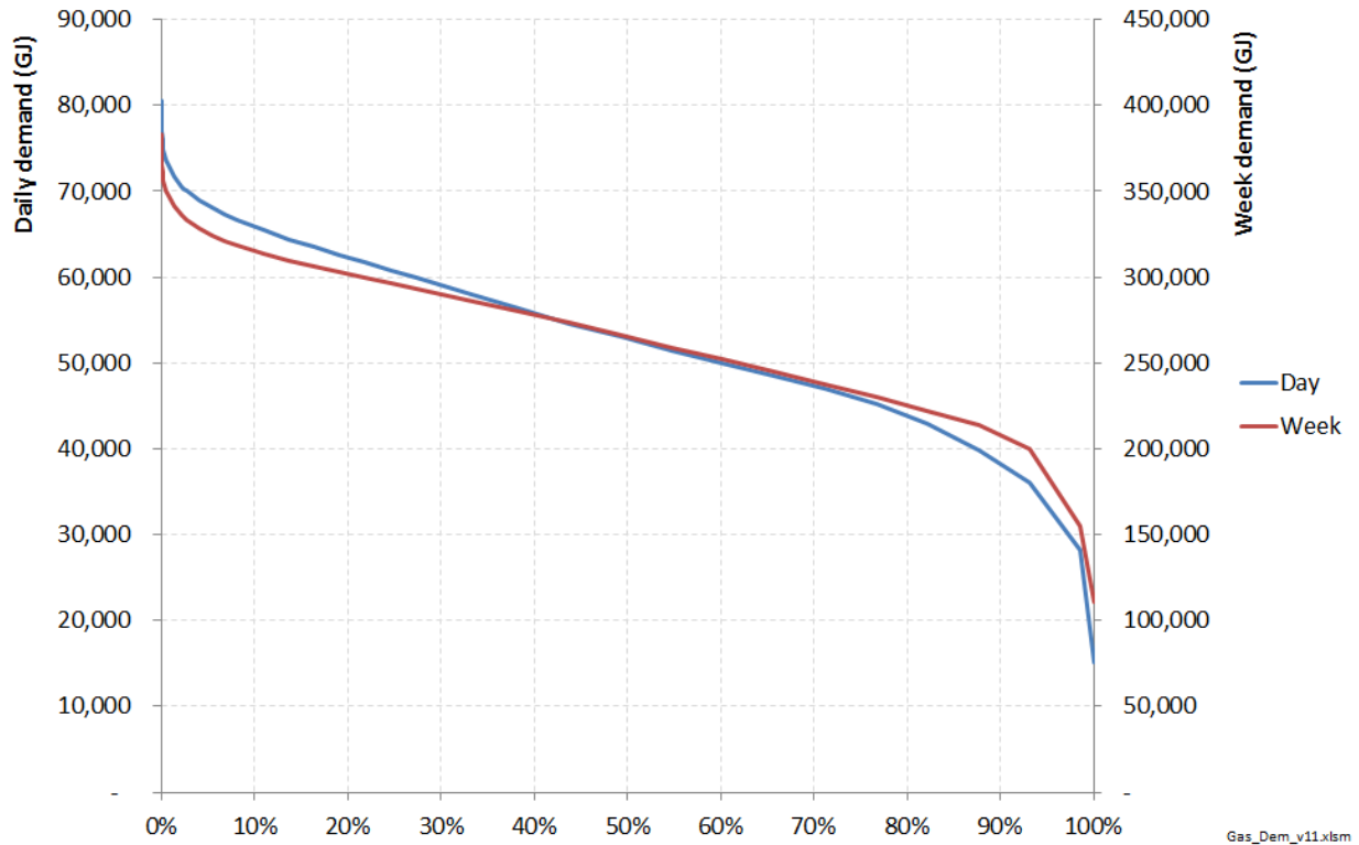
Figure 60: Modelled duration curves of non-generation demand on the North System
