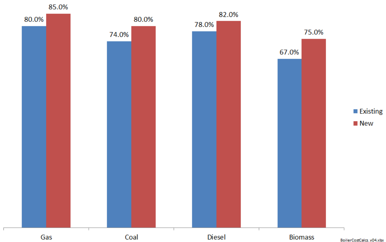
Figure 80: Average intermediate process heat boiler efficiencies
