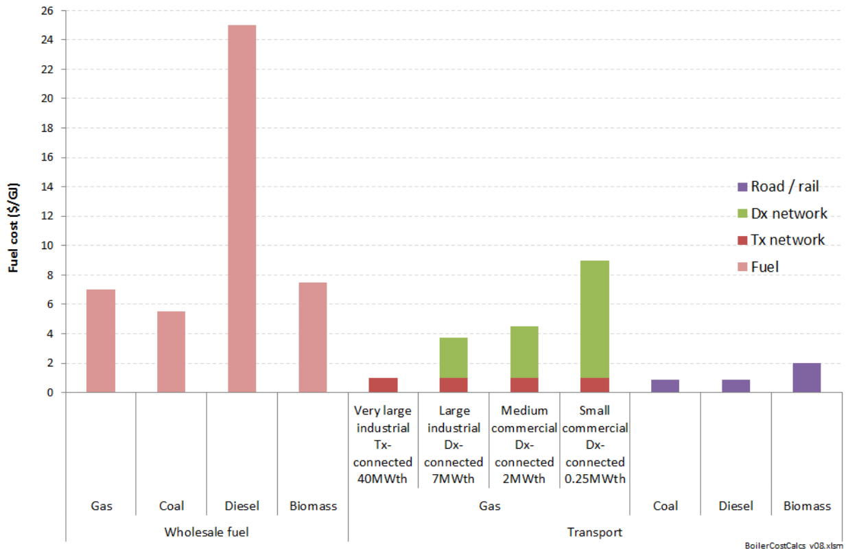
Figure 81: Fuel and transport costs for different boiler options
